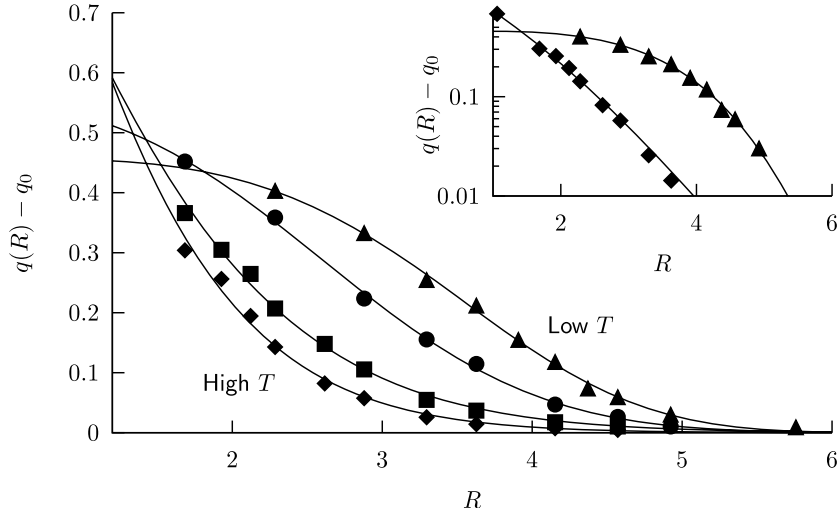
Figure 1. Point-to-set correlation (overlap) versus cavity radius for the soft-sphere binary mixture at temperatures T = 0.482 (diamonds), 0.350 (squares), 0.246 (circles), and 0.203 (triangles) [4]. Lines are fits to the compressed exponential form (18). Inset: same data for the highest and lowest temperatures in log-linear scale, showing the non-exponential character of the overlap decay at low temperatures (an exponential shows as a straight line in this plot).
