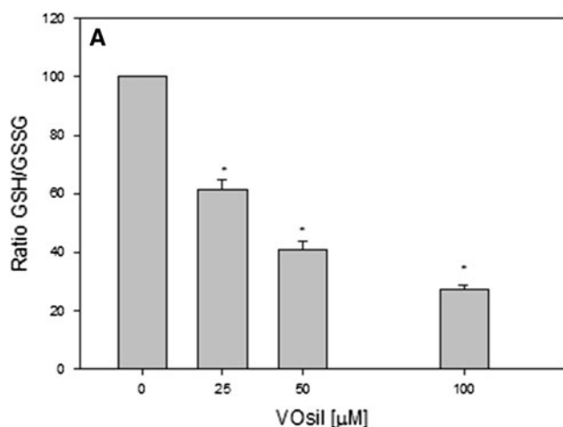
Fig. 9 a Ratio of reduced glutathione ( GSH ) to oxidized glutathione ( GSSG ) in MG-63 cells incubated with different concentrations of VOsil. The results are expressed as the mean \pm SEM of three independent experiments. Asterisk significant differences versus the basal level ( p < 0.01 ). b Effect of VOsil on MG-63 cell viability in
