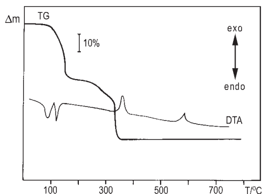
Fig. 2 TG and DTA curves of \text{Li}_3(\text{Cit}) \cdot 5\text{H}_2\text{O}
