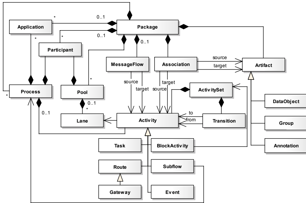
Figure 5. XPDL partial metamodel.
