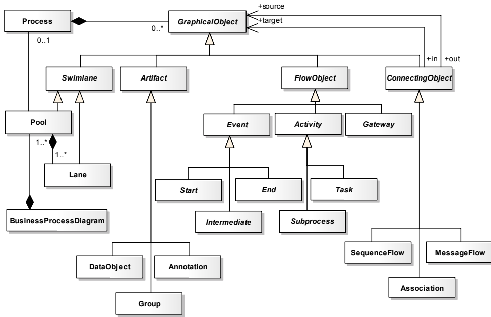
Figure 4. BPMN partial metamodel.
