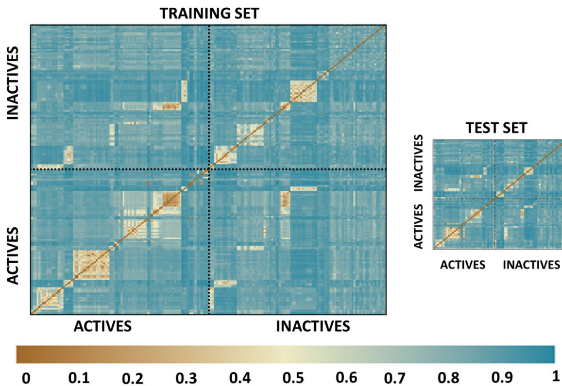
Supplementary Fig. 1 Dissimilarity heatmaps for the training and test sets. Saddle brown areas indicate high similarity between the compared pair of compounds, while Steel blue areas indicate low similarity between the compared compounds
