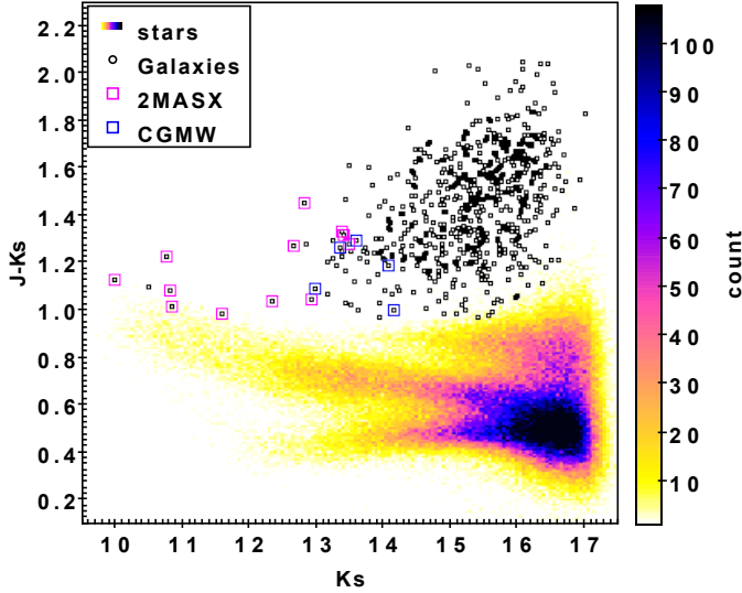
Fig. 9: J-Ks vs. Ks total magnitude diagram. Circles correspond to galaxy candidates. Galaxies catalogued by other surveys are shown by squares. The density map shows the distribution of stars and the colour scale corresponds to number counts, as shown in the key.
