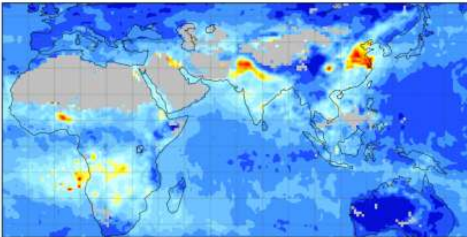
ol Optical Thickness at 0.55 microns for both Ocean (best) and Land (corrected): Mean of Daily Mean (
