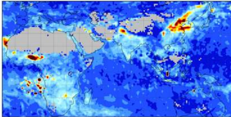
ical Thickness at 0.55 microns for both Ocean (best) and Land (corrected): Standard Deviation of Daily
