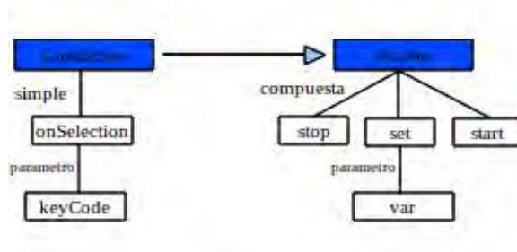
Figura 18: Conector onKeySelectionStopSetStart
