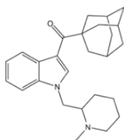
I.4- adamantoil -indol
