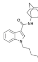
I.7- APICA (indol-carboxamida)
