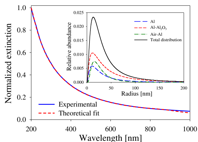
Fig. 10 Experimental extinction spectrum of Al NPs fabricated by laser ablation in water (full line) with 500 \mu J pulse energy. Theoretical fit (dashed line) using Mie theory with the size-dependent metal dielectric function determined in this work. The inset shows the species size distribution derived from the optimum fit
