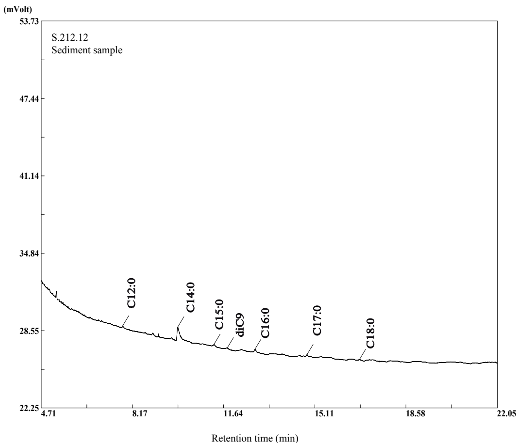
Supplementary Figure A: Chromatograms obtained by GC-FID of fatty acid methyl esters (FAMES) recovered in sample EC.212.12 ( Santa María jar), and sample S.212.12 (sediment adhered to the internal surface of EC.212.12), from El Colorado, Catamarca, Argentina.
