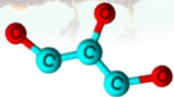
Glicerol
