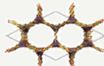
CPO-27 (X)
