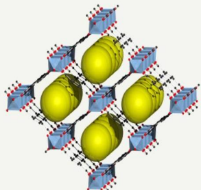
MIL-53 (X)
