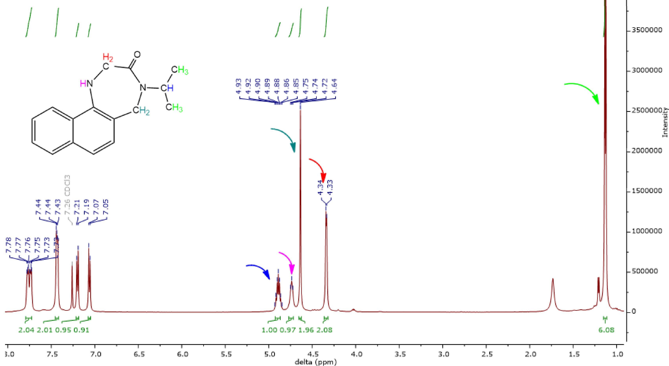
1 H RMN 1,2,4,5-tetrahydronaphtho[1,2-e]-4-isopropyl-1,4-diazepin-3-one spectra
