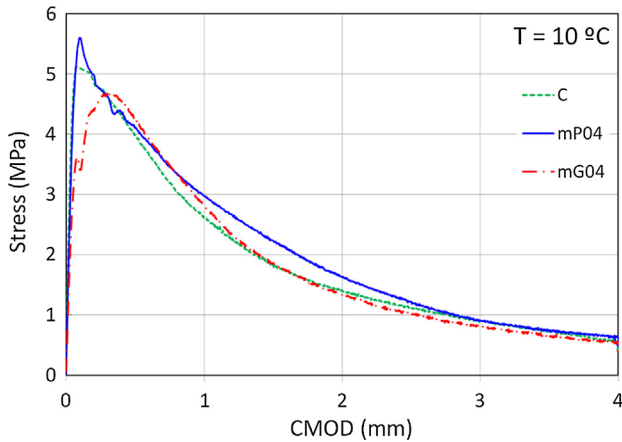
Fig. 7. Stress – CMOD curves of FRAC incorporating microfibers.
