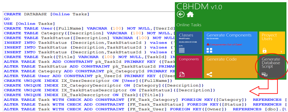
Fig. 3. Generating Database Script from UI Model
