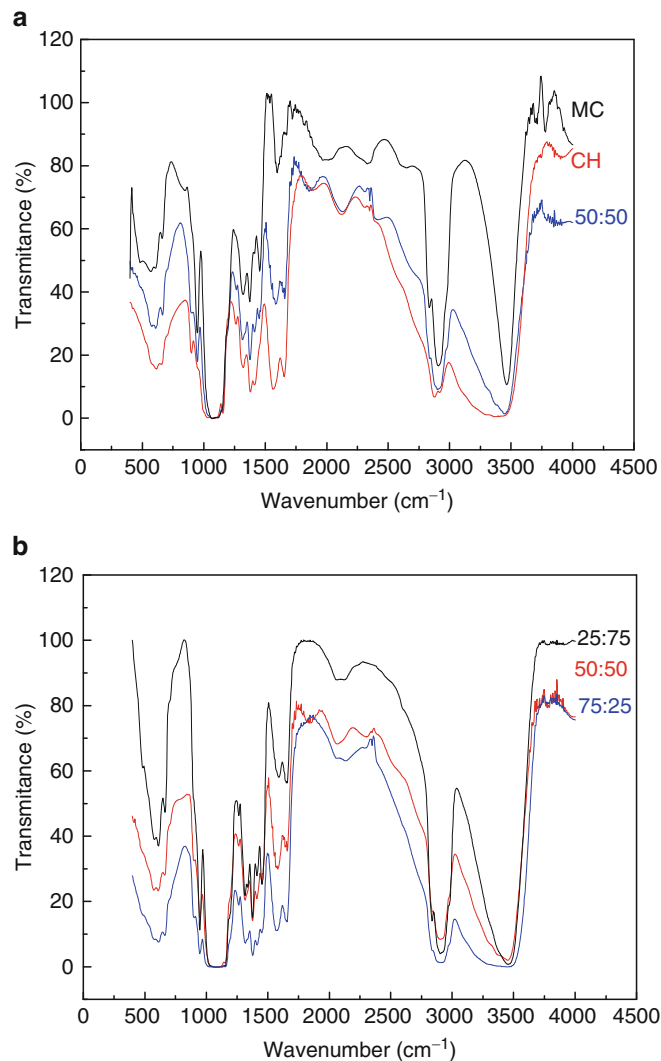
Fig. 6.6 FTIR characterization of: (a) MC, CH and 50:50 films and (b) composite films with different CH:MC ratios
