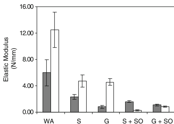
Fig. 6.11 Tensile properties: elastic modulus of corn ( open rectangle ) and amylomaize ( filled dot ) films (WA = without additives; S = with sorbitol; G = with glycerol; S + SO = with sorbitol and sunflower oil and G + SO = with glycerol and sunflower oil)
