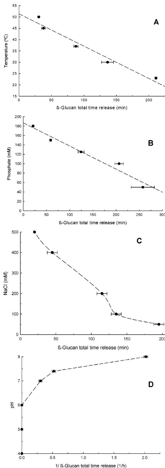
Figure 8. Effect of temperature in 100 mM phosphate buffer (pH 7.4) (A), phosphate concentration (pH 7.5) at 37 °C (B), NaCl in 50 mM phosphate buffer (pH 7.4) (C), and pH in McIlvaine or phosphate buffers (125 mM) at 37 °C (D) on the amount of \beta -glucan released from emulsan-coated microspheres.
