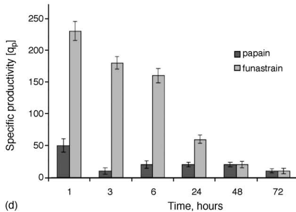
Fig. 4. Comparison of funastrain and papain specific productivities [ q_p = nmoles of Z-Ala-Phe-OMe/enzyme unit × h] during the reaction course. (A) Equilibrium-controlled synthesis in acetonitrile of a_w \cong 0.12 ; (B) kinetic-controlled synthesis in acetonitrile of a_w \cong 0.12 ; (C) equilibrium-controlled synthesis in ethyl acetate of a_w \cong 0.75 ; (D) kinetic-controlled synthesis in ethyl acetate of a_w \cong 0.75 .
