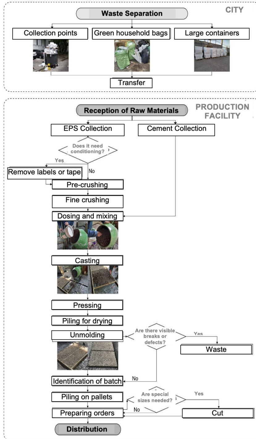
Figure 1. Flow diagram of the alternative thermal insulation board production process. Source: Preparation by the authors.
