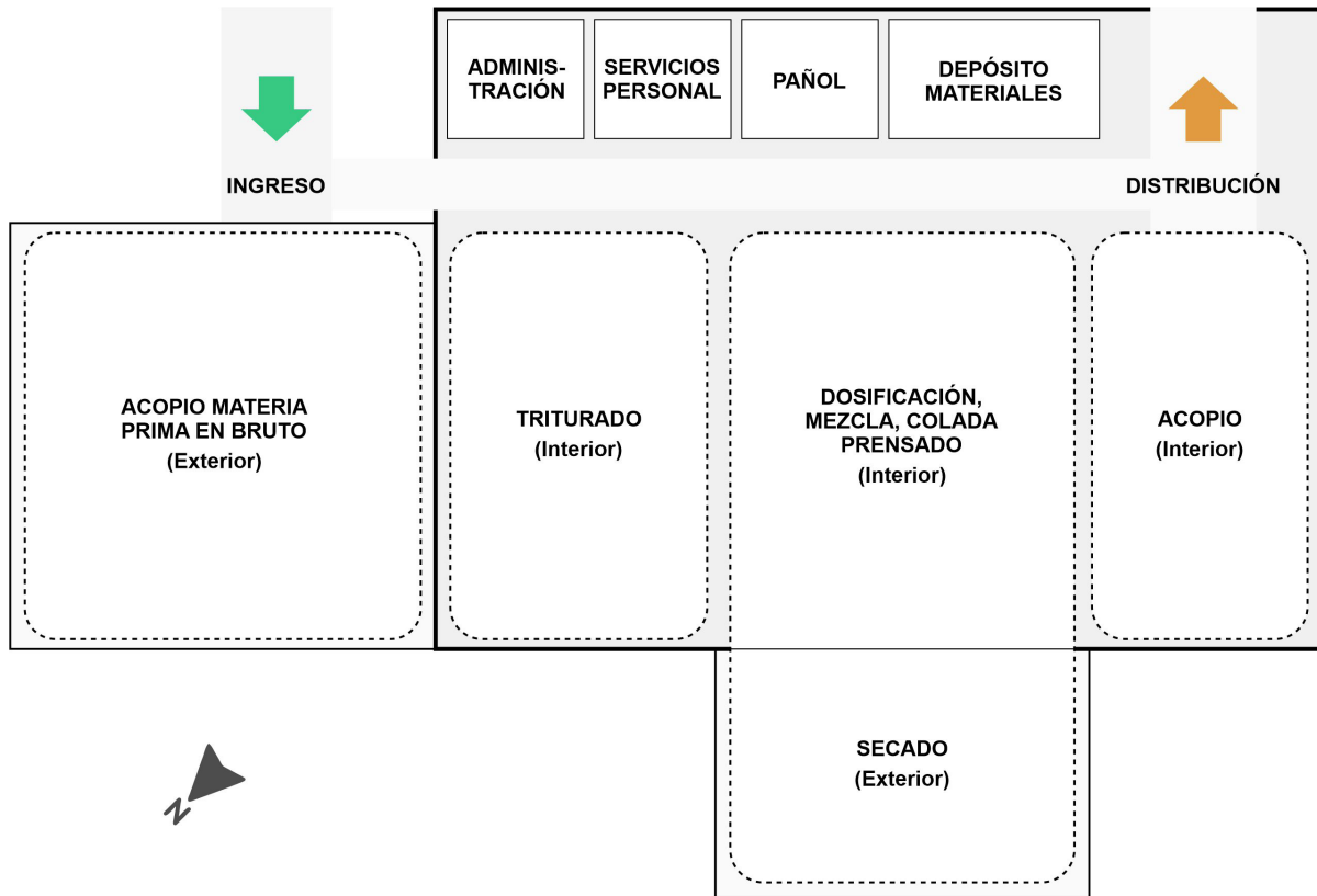
Figure 5. The organizational layout of the production facility. Source: Preparation by the authors.
