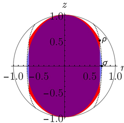
Figure 2. Projection of the Bloch sphere on the z - r plane. The black dots represent two qubit states: \rho (upper dot, with r_1 = 0.69135 , z_1 = 0.5 ) and \sigma (lower dot, with r_2 = 0.732828 , z_2 = 0 ). The red and blue regions represent the projection of the sets \{\rho' : \rho \xrightarrow{\text{IO}} \rho'\} and \{\rho' : \sigma \xrightarrow{\text{IO}} \rho'\} on the z - r plane, respectively. The dotted black curve represents the set \{\rho' : C_{\text{re}}(\rho') = 0.3\} projected on the z - r plane. From the figure, it can be observed that \rho and \sigma are IO-incomparable, and C_{\text{re}}(\rho) = C_{\text{re}}(\sigma) = 0.3 .
