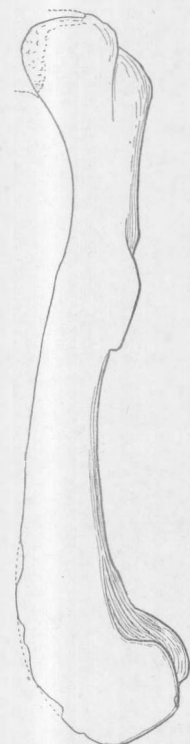
Fig. 52. — As 47. Anterior aspect of right femur, in \frac{1}{2} nat. size.
