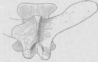
Fig. 5. — Anterior caudal vertebra from above in \frac{1}{2} nat. size. From Stonesfield, in the Oxford Museum. Specimen already figured by Buckland etc., in other views.
