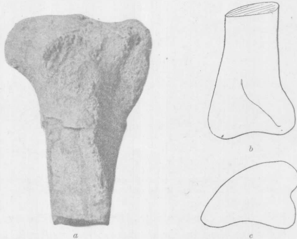
Fig. 34. — Proximal half of right tibia with crista lateralis : a , in lateral view in slightly less than \frac{1}{2} nat. size ; b , distal extremity of the same in anterior view, \frac{1}{4} nat. size ; c , outline of proximal end of left tibia from above in \frac{1}{4} nat. size.
