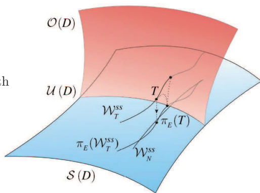
FIGURE 2. The projection argument
