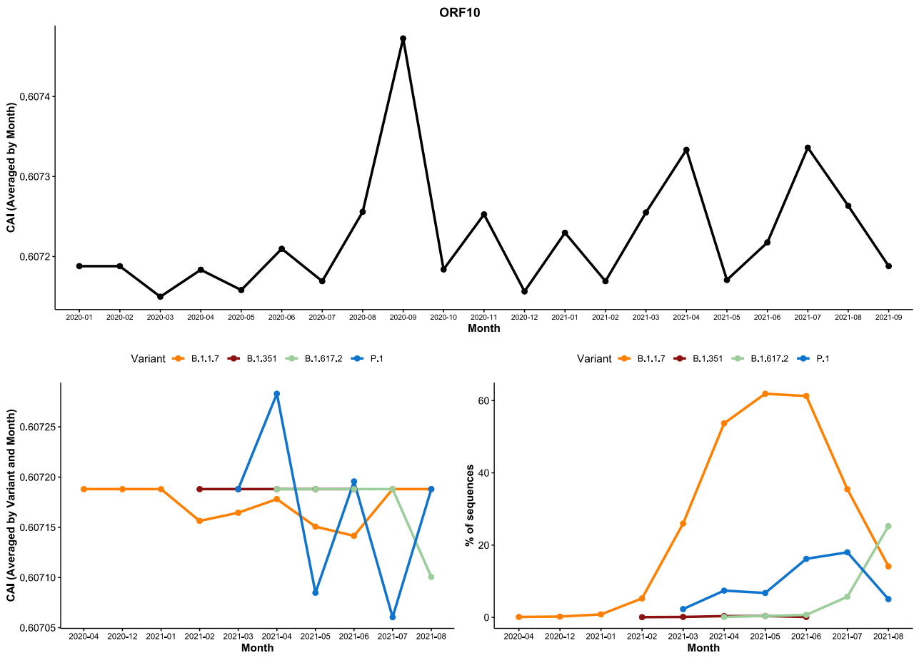
Figure S16. Evolution of CAI for SARSCoV2 ORFs over time for the California dataset.
