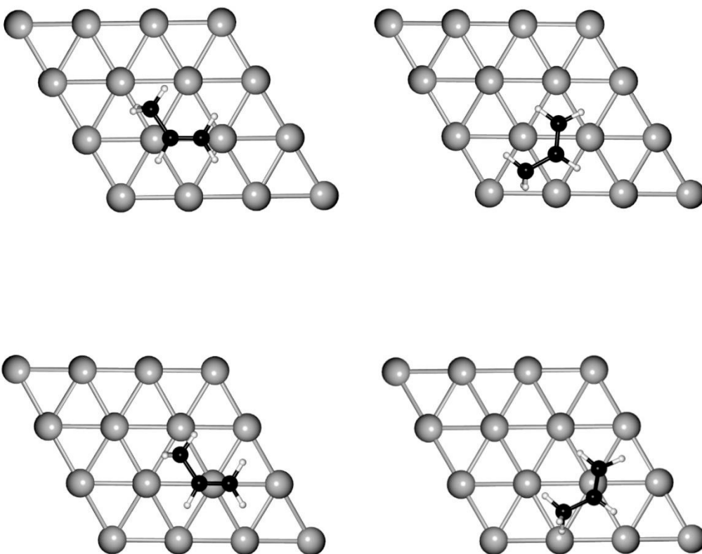
Figure S2. initial geometries for optimization calculations of propene adsorption over Ag(111).
