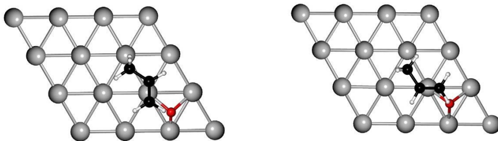
Figure S3. initial geometries for optimization calculations of propene adsorption over Ag(111) with a O adatom.
