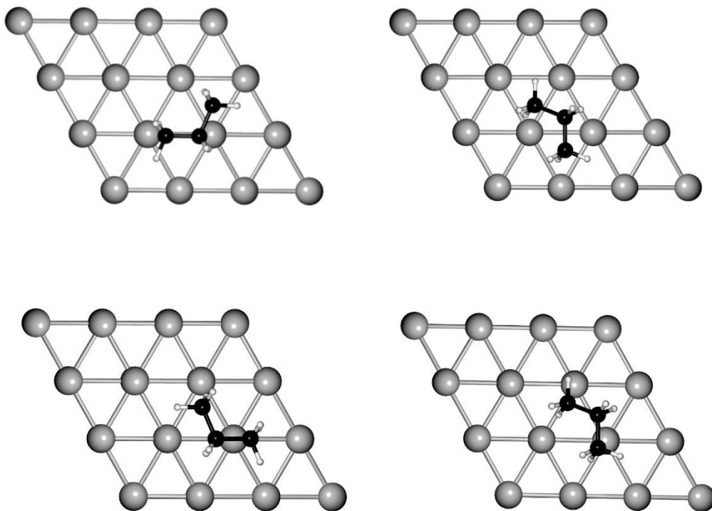
Figure S1. initial geometries for optimization calculations of propane adsorption over Ag(111).
