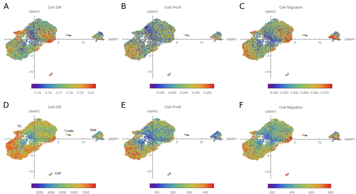
Figure S1: UMAP representation of the TNBC sample (TN-0135) assessing three biological processes: cell differentiation, cell population proliferation and cell migration. A-C: Cells are colored by the PPIN activity (ORIGINS2) associated with the corresponding biological process. D-F: Cells are colored by the AUCell score corresponding to the gene set of the biological process in question.
