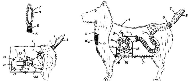
ANNE MARGARET ZALESKI COMBINATION TOY DOG AND VACUUM CLEANER Patented November 13, 1973 No. US 3,771,192
