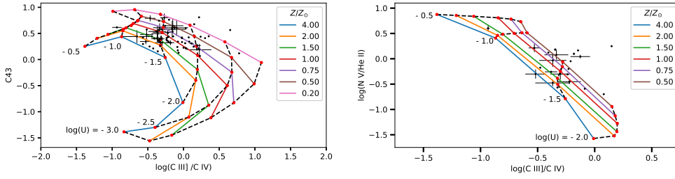
Figure 1. On the left panel, the grid composed by \log(\text{C III}] \lambda 1909/\text{C IV} \lambda 1549) and C43 line ratios, and, on the right panel, it shows one with \log(\text{C III}] \lambda 1909/\text{C IV} \lambda 1549) and \log(\text{N V} \lambda 1240/\text{He II} \lambda 1640) line ratios.
