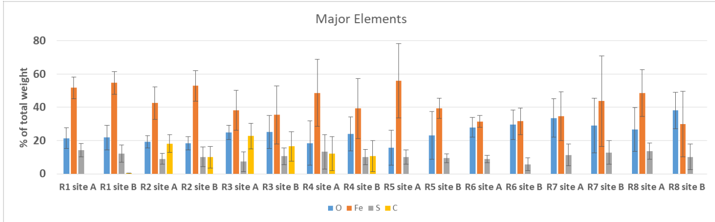
Figure S2. EDX graph. Two sites (labeled as site A and site B) were selected for each coupon for EDX analysis. Two 1\ \mu\text{m} \times 1\ \mu\text{m} scan areas per coupon were examined, with 4 to 7 points examined in each scan area. In total, 8 to 14 spectra were obtained for each coupon. The % weight of oxygen, iron, sulfur and carbon was plotted below as the mean value and \pm 1 STD error bars. R1, R2: petro-F76. R3, R4: FT-F76. R5, R6: fuel mix. R7, R8: no fuel.
