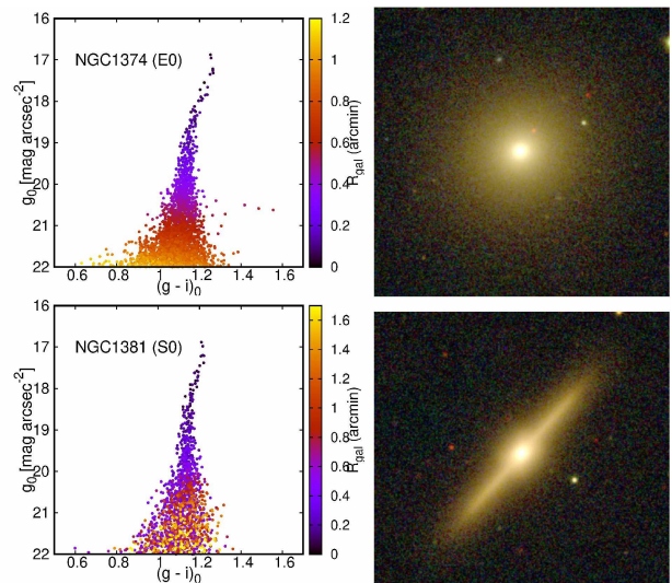
Figure 4: Top left panel: pixel color-magnitude diagram of the galaxy NGC 1374 shown in the top right panel . Bottom left panel: pixel color-magnitude diagram of the galaxy NGC 1381 shown in the bottom right panel . Due to the similarities between the pCMDs of both galaxies, we wonder if NGC 1374 could be a face-on S0 misclassified as E as a consequence of an inclination effect.
