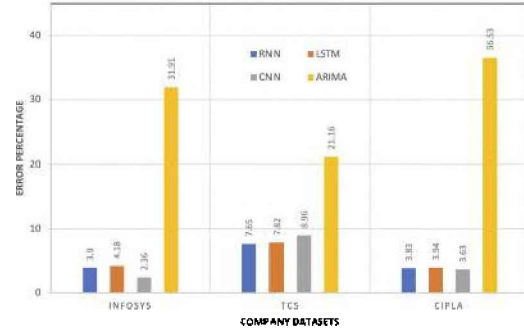
PERFORMANCE OF SLIDING WINDOW VS. DEEP LEARNING METHODS
