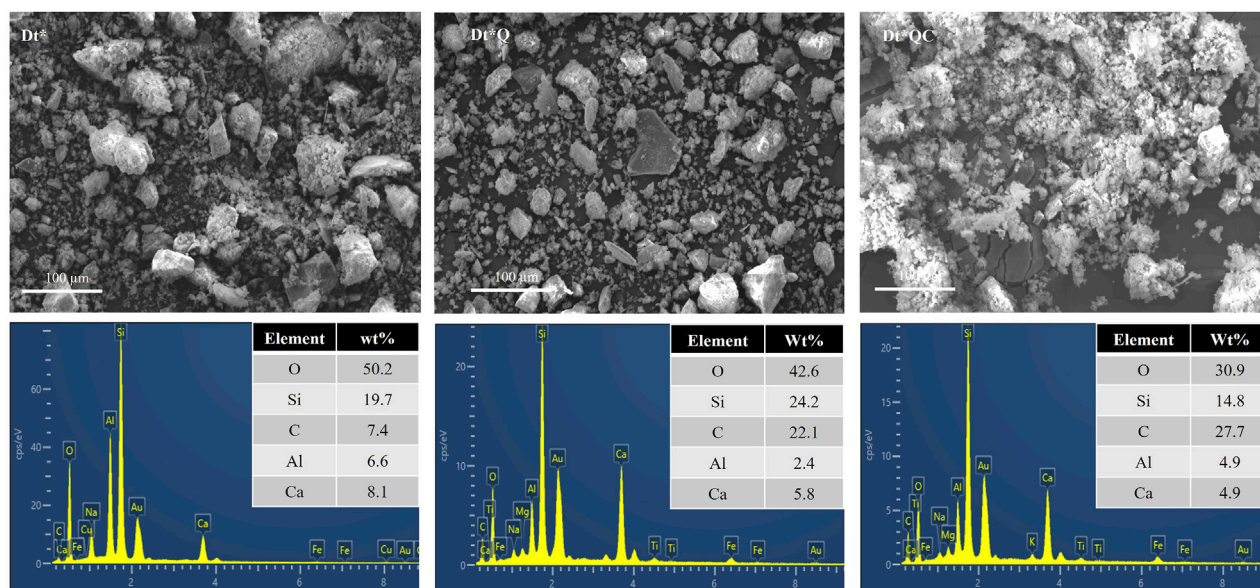
FIGURE 5 SEM micrographs (magnification \times 500 ) and EDS elemental surface analysis: Dt*, Dt*Q, and Dt*QC.
