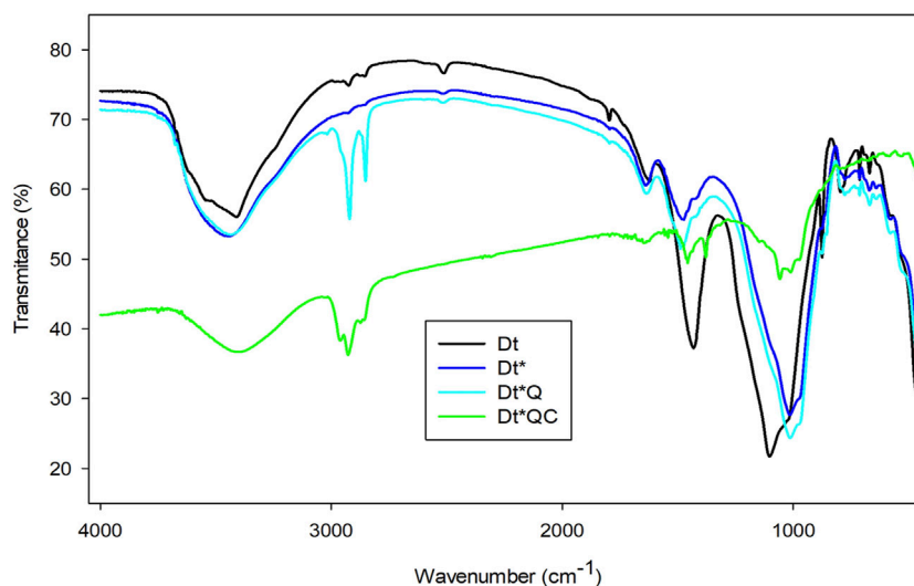
FIGURE 6 FTIR spectra: Dt, Dt*, Dt*Q, and Dt*QC.
