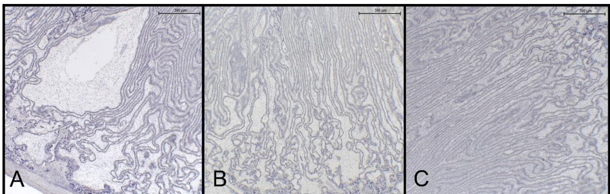
Figure 2. Negative controls for the immunohistochemical detection of (A) IGF1R, (B) IGF1, and (C) IGF2 in the feline placenta. IHC. DAB. (Bar=500 \mu m).
