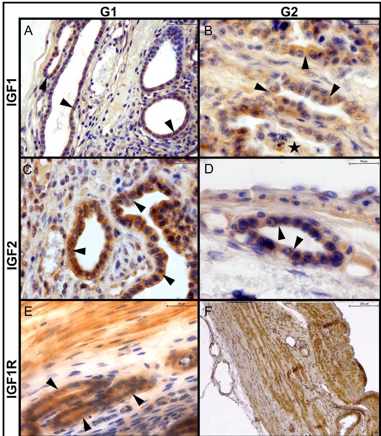
Figure 3. Feline placenta. Immunohistochemical detection of IGF1, IGF2, and IGF1R in the maternal zone, in samples from groups 1 (G1) and 2 (G2). Cytoplasmic labelling of the three molecules (A) IGF1, G1. Strong labelling in glandular cells (arrowheads (Bar=100µm)). (B) IGF1, G2. Histotroph (stars) and glandular cells are moderately labeled (Bar=50µm). (C) IGF2, G1. Strong labelling in glandular cells (Bar=50 µm). (D) IGF2, G2. Moderate labelling in glandular cells (Bar=50 µm). (E) IGF1R, G1. Strong labelling in glandular cells (Bar=50 µm). (F) IGF1R, G2. Strong labelling in myometrial myocytes (Bar=200µm). Arrowheads: glandular cells; stars: histotroph. IHC. DAB.
