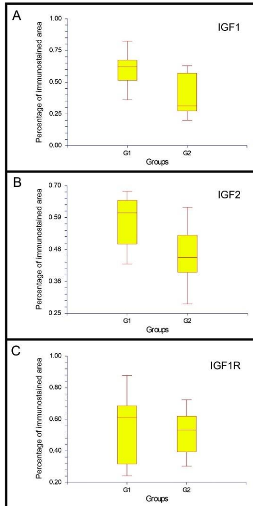
Figure 6. Percentage of the immunostained area in the placenta and gravid uterus of the cat. P values for the differences between groups 1 and 2 were: p = 0.00000001 ; n=10 for IGF1 (A), p = 0.0002 ; n=10 for IGF2 (B), and p=0.1558 ; n=10 for IGF1R (C).
