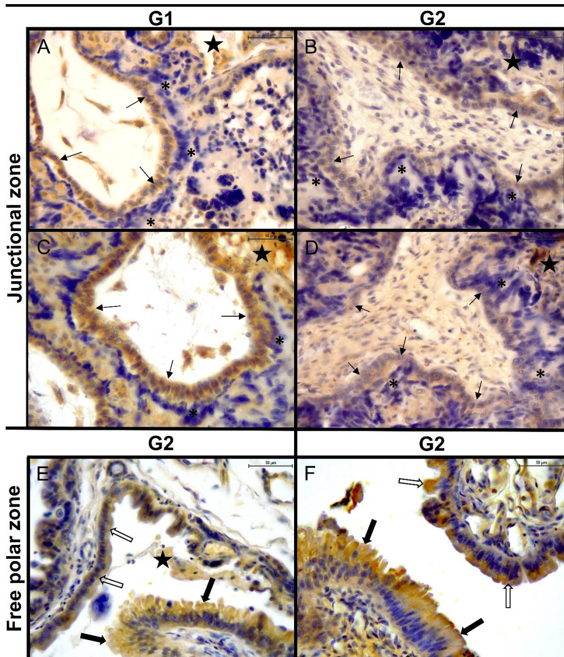
Figure 5. Feline placenta. Immunohistochemical detection of IGF1, IGF2, and IGF1R in the junctional zone (JZ) and the free polar zone. (A) JZ. IGF1, G1. Strong labelling in the JZ-CTB (thin arrows) and the histotroph (black stars). The labelling in the JZ-STB (asterisks) was inconsistent (negative in this image). (B) JZ. IGF2, G2. Moderate labelling in JZ-CTB and histotroph. The JZ-STB was negative. (C) JZ. IGF1R, G1. Strong labelling in JZ-CTB and histotroph. The JZ-STB was negative. (D) JZ. IGF1R, G2. Moderate labelling in JZ-CTB and histotroph. The JZ-STB was negative. (E) Free polar zone. IGF1, G2. Moderate labelling in the uterine epithelium (thick empty arrows), the trophoblast (thick black arrows), and the histotroph. (F) Free polar zone. IGF1R, G2. Moderate labelling in the uterine epithelium and the trophoblast. Thin arrows: cytotrophoblast of junctional zone (JZ-CTB); asterisks: syncytiotrophoblast of junctional zone (JZ-STB); black stars: histotroph; thick empty arrows: uterine epithelium; thick black arrows: trophoblast (TB). IHC. DAB. (Bar=50 \mu m).
