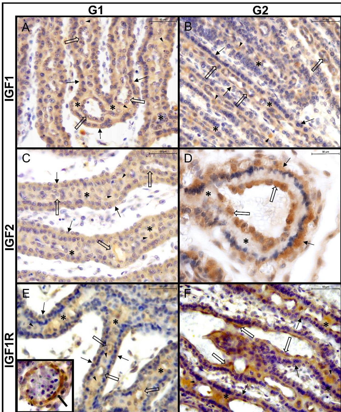
Figure 4. Feline placenta. Immunohistochemical detection of IGF1, IGF2, and IGF1R in the labyrinth, in samples from groups 1 (G1) and 2 (G2). (A) IGF1, G1. Moderate labelling in CTB (thin arrows) and maternal endothelium (thick empty arrows). DC (arrowheads) and STB (asterisks) were mildly labelled. (B) IGF1, G2. Mild labelling in CTB and STB, moderate in DC, and strong in the maternal endothelium. (C) IGF2, G1. Moderate labelling in CTB, maternal endothelium, and DC. Mild labelling in STB. (D) IGF2, G2. Moderate labelling in CTB, mild labelling in STB. Maternal endothelium is strongly labelled. (E) IGF1R, G1. Moderate labelling in CTB and STB. Mild labelling in DCs and strong in the maternal endothelium. Inset: strong labelling in the endothelium of a fetal vessel. (F) IGF1R, G2. Mild labelling in CTB and STB. The DCs are moderately labelled. Strong labelling in maternal endothelium. Thin arrows: cytotrophoblast (CTB); black arrowheads: decidual cells (DC); asterisks: syncytiotrophoblast (STB); thick empty arrows: maternal endothelium; thick black arrow: fetal vessel. IHC. DAB. (Bar=50 µm).
