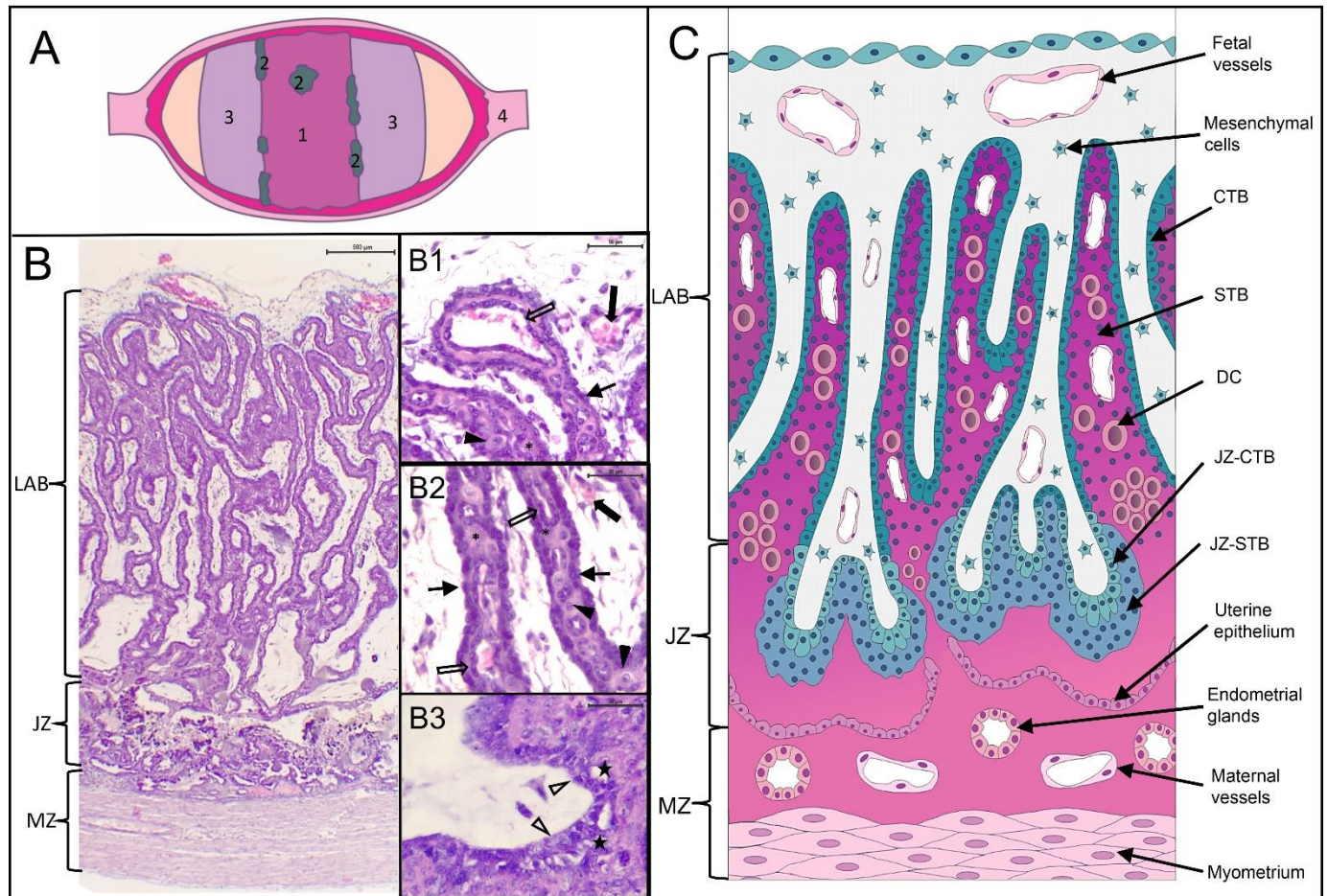
Figure 1. Feline placenta. (A) Schematic diagram of the placental gross appearance (cut surface of the uterus). 1. Placental girdle; 2. Hematophagous organs; 3. Free polar zones; 4. Interplacental uterine site. (B) Structure of the feline placenta. Hematoxylin and eosin (HE). Laminar arrangement of maternal and fetal structures (Bar=500 \mu m). (B1, B2, B3) magnification of B. (B1) Fetal zone (Bar=50 \mu m). (B2) Labyrinth (Bar=50 \mu m). (B3) Junctional zone (Bar=50 \mu m). LAB: labyrinth; JZ: junctional zone; MZ: maternal zone; thin arrows: cytotrophoblast (CTB); asterisks: syncytiotrophoblast (STB); black arrowheads: decidual cells (DC); thick empty arrows: maternal endothelium; thick black arrows: fetal vessels; empty arrowheads: JZ-CTB; black stars: JZ-STB. (C) Schematic representation of the placental girdle showed in (B) .
