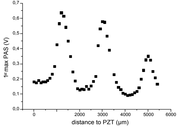
Figure 4: The centers of clear bands and black grooves are clearly resolved by scanning the surface with the laser. The signals were taken at 100\text{ }\mu\text{m} displacement from each other. The energy of PAS decreases with distance of the laser beam to PZT. The increment in signal due to the grooves is more than 6-fold with respect to the signal due to the bulk polymer.
