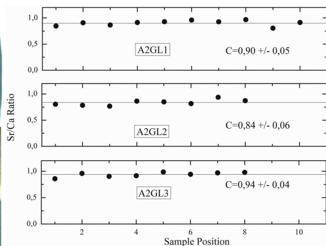
Fig. 4 - a) Laser dots along two growing lines in the buccal aspect of A1 lower M3. b) Laser dots along two growing lines in the buccal aspect and one growing line in the lingual aspect of A2 lower M3. Numbers in dots refer to Sr/Ca ratios shown in the plot on the right. It is worth noting that incremental lines were followed in areas in which maps revealed that Sr/Ca ratios are more or less stable.
