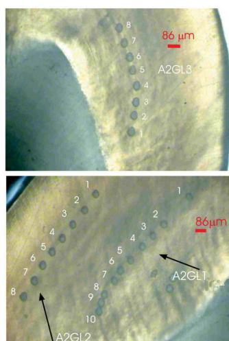
Fig. 4 - a) Laser dots along two growing lines in the buccal aspect of A1 lower M3. b) Laser dots along two growing lines in the buccal aspect and one growing line in the lingual aspect of A2 lower M3. Numbers in dots refer to Sr/Ca ratios shown in the plot on the right. It is worth noting that incremental lines were followed in areas in which maps revealed that Sr/Ca ratios are more or less stable.
