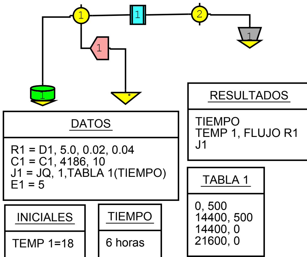
Figure 2: A thermal circuit, drawn with Dia
