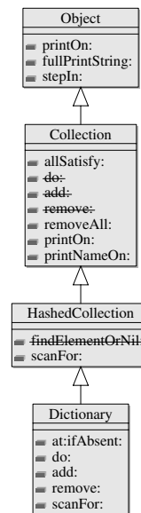
Fig. 2. Initial Code Base.
