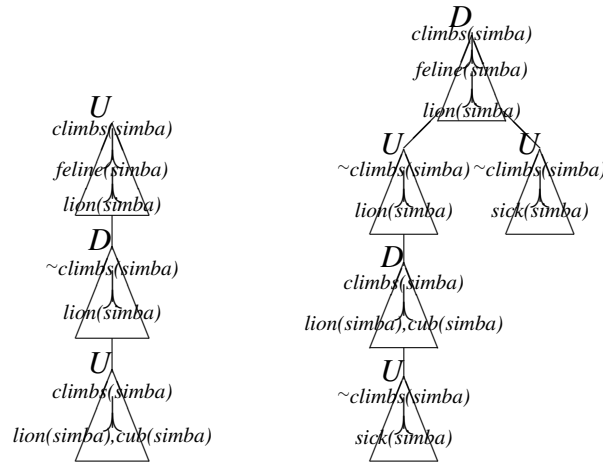
Figure 2: First and second dialectical trees from Example 3.1
