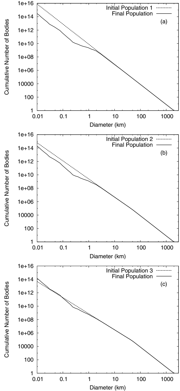
Fig. 4. Our estimates of the Plutino cumulative size distribution after 4.5 Gyr of evolution obtained from the different initial populations proposed in Sect. 4.
