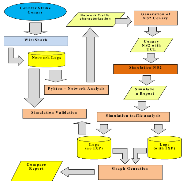
Figure 7. NS2 Methodology
