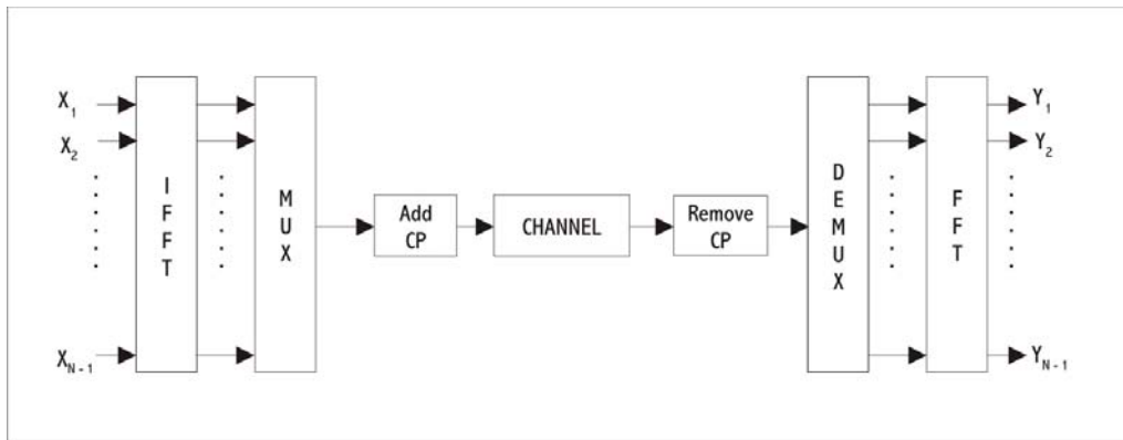
Figure 5: OFDM Diagram
