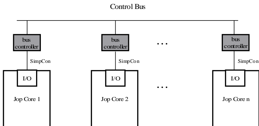
Figure 3.1 The control bus. The bus controller I/O device is used to provide access to a common control bus shared among all the processors.
