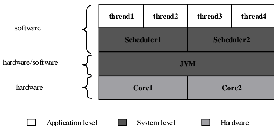
Figure 4.1 Overall architecture of a dual core JVM with two independent schedulers. Each application is written as a set of threads. Each thread is then “tied” to a specific scheduler which runs on one processor. JVM code is accessed by scheduler 1 and scheduler 2 and is thus executed on both cores.
