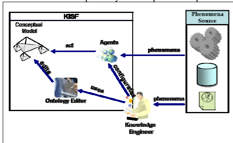
Figure 1 - KISF Architecture
