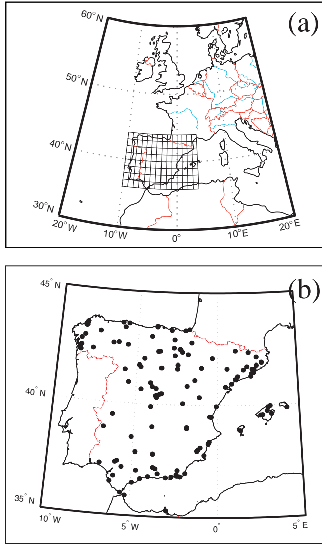
Figure 1: (a) High resolution limited area grid with 1.0^\circ (approx. 80 Km) for both latitude and longitude. (b) Primary network of 112 climatic stations of the INM.
