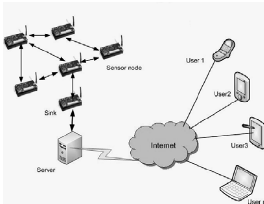
Fig. 1. System Architecture of the deployed testbed
