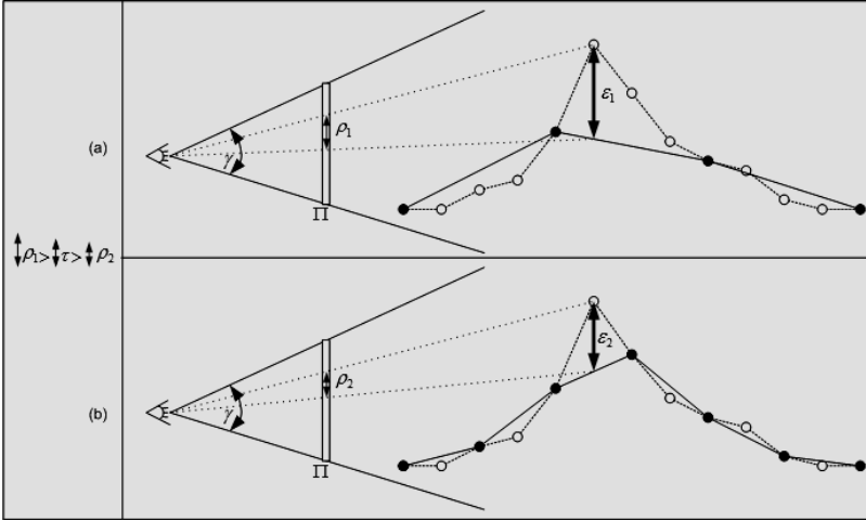
Fig. 2. World-space errors \varepsilon_1 and \varepsilon_2 , originated from two different LOD representations, are projected into the projection plane \Pi . (a) Level 2 representation: maximum screen-space error \rho_1 exceeds threshold \tau . (b) Level 1 representation: maximum screen-space error \rho_2 is smaller than threshold \tau
