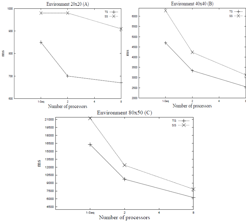
Fig. 10. EVAC*: Parallel Simulation Time
