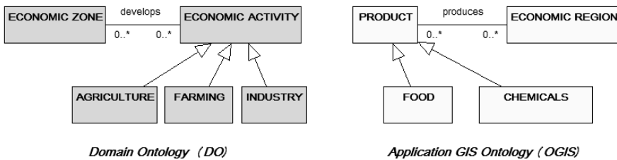
Fig. 3. DO ontology and OGIS application ontology relationship
