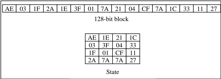
Fig. 1. AES State
