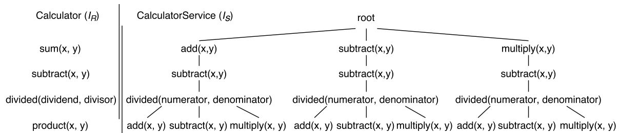
Figure 3: Wrapper generation tree to Calculator Service
