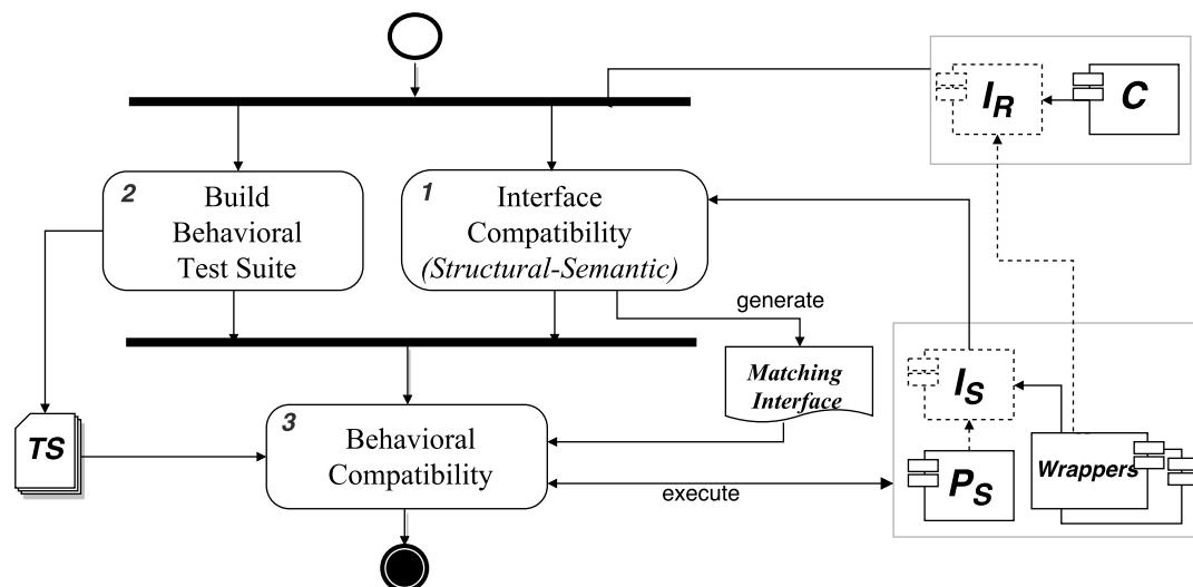
Figure 1: Service Selection Method
