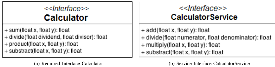
Figure 2: Case Study of Calculator service
