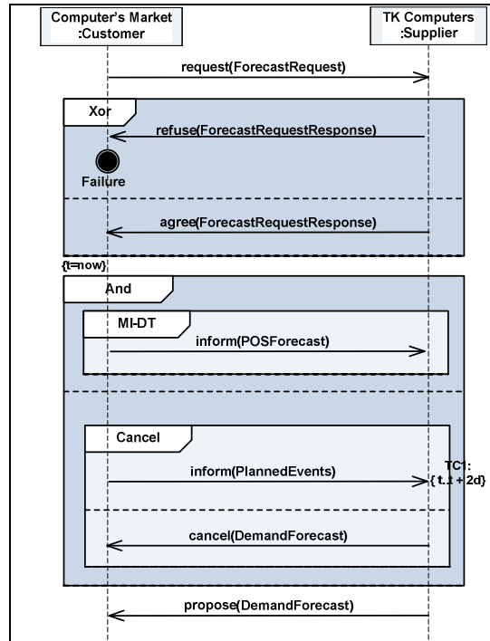
Fig. 2. Collaborative Demand Forecast CBP model defined with UP-ColBPIP
