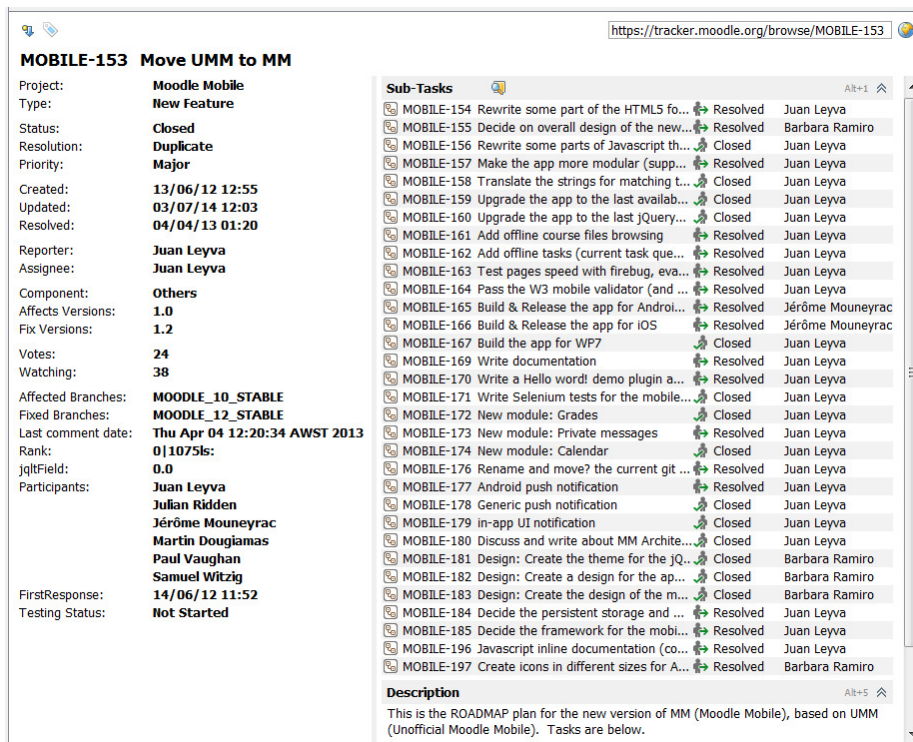
Fig. 11. Issue MOBILE-153.
