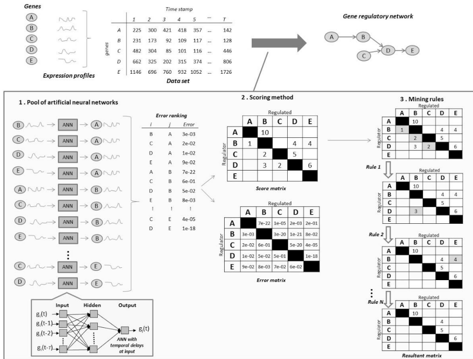
Figure 1. GRNNminer: a three steps approach for discovering relations between variables (genes) from time series (expression profile).
