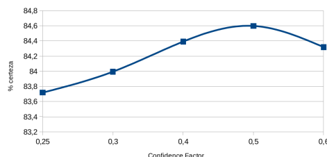
Figura 2. Confidence factor
